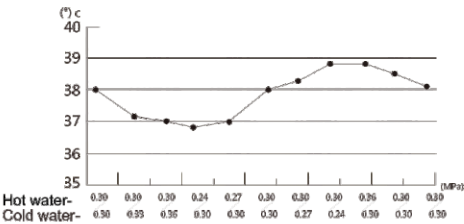
Supply water pressure vs outlet water temperature
