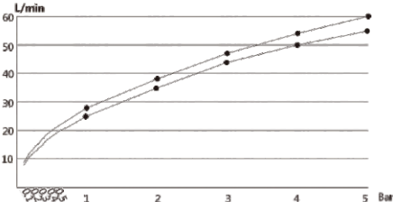
Supply water pressure vs outlet flow rate
